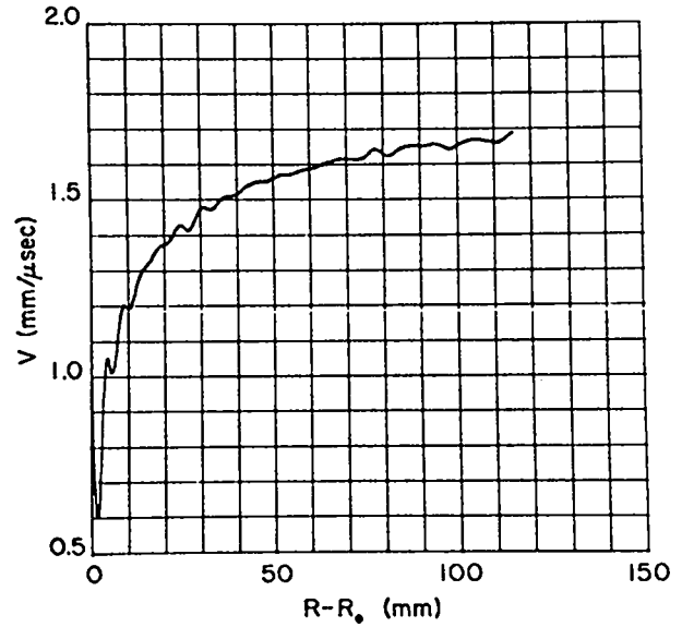
Fig. A-1. Velocity vs expansion radius for the 101.4-mm Comp. B cylinder test. A forty-knot spline fit was used in the data reduction. The explosive density was 1.701 g/cm 3 and the loading factor 4.0331 g/cm 3 .
